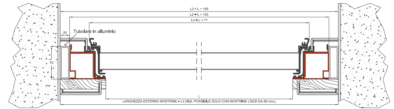
Soluzione 5 - Porta blindata montata tra due muri Solution 5 - Armoured door mounted between two walls
